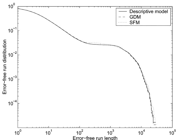
Fig. 1. EFRDs of the generative models and the descriptive model.
