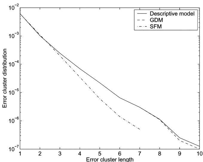
Fig. 2. ECDs of the generative models and the descriptive model.
