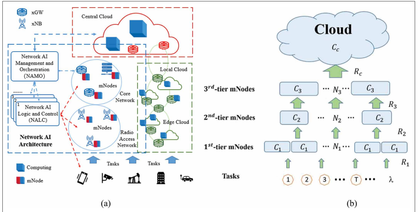
FIGURE 2. Three AI architectures and the system model. a) Deployments of cloud, edge, and network AI architectures. b) System model.
