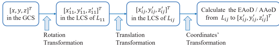
Fig. 5. Flow chart of calculating angles in the LCS of L_{ij} .
