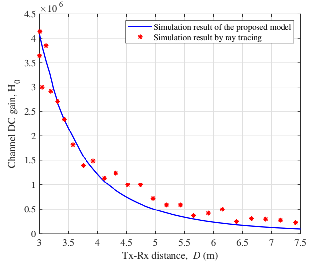
Fig. 9. Channel DC gains of the proposed channel model and the ray tracing results in [30] ( \sigma_{DS} = \sigma_{AS} = 1.2 m, \sigma_{ES} = 1 m, N_{c,\text{total}} = 25 , N_{c,\text{SB}} = 22 , A_{c,\text{eff}} = 5 m 2 , v^R = 1 m/s, \alpha_A^R = 0 , \alpha_E^R = \frac{\pi}{2} , D = 3 m, t = 0 - 7 s).
