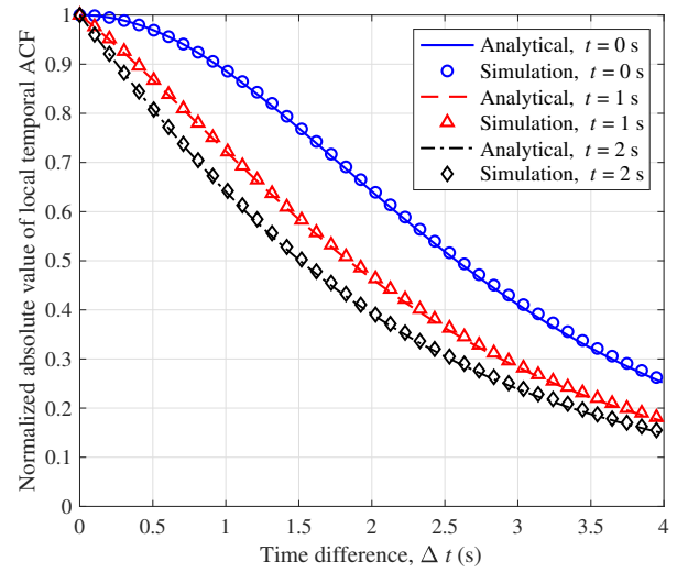
Fig. 6. Temporal ACFs at different time instants (sub-channel: L_{11} -PD, v^R = 0.5 m/s, \alpha_A^R = 0 , \alpha_E^R = \pi/2 , \sigma_{DS} = \sigma_{AS} = \sigma_{ES} = 1 m, \lambda_B = 80 /m, \lambda_D = 4 /m, D_C^A = 10 m).
