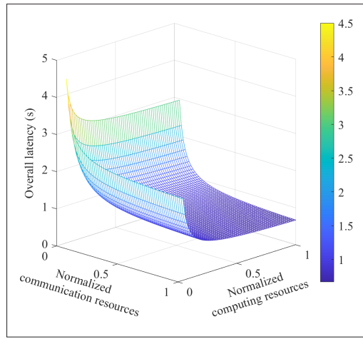
FIGURE 2. A schematic diagram of the overall latency of a single offloading task with different communication and computing resources provided.
