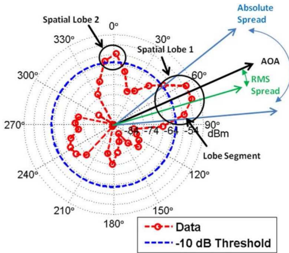
Fig. 8. Measured PAS where two SLs have a -10 dB power threshold [70].
