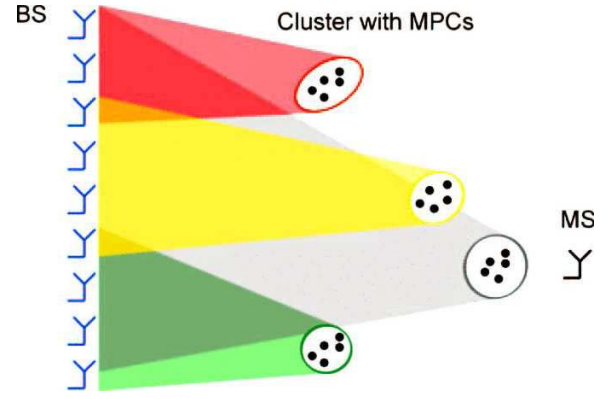
Fig. 3. Extension of cluster visibility regions to the base station side [81].
