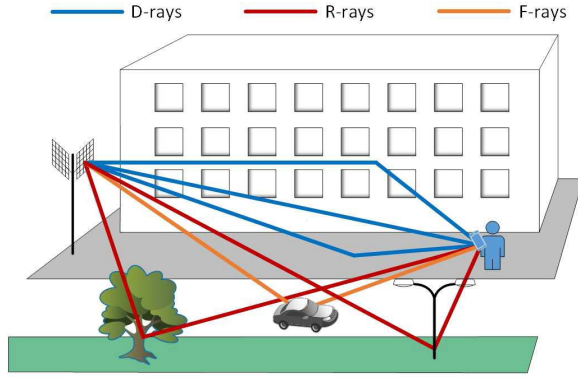
Fig. 14. D-rays, R-rays, and F-rays in IEEE 802.11ay channel model [202].
