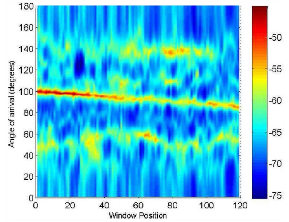
Fig. 1. APSs over the array in the LoS case [21].
