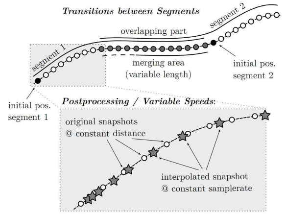
Fig. 11. Transitions between segments and obtaining the velocity variations by interpolation [198].
