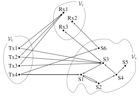
Fig. 6. A propagation graph with four transmit vertices, three receive vertices, and six scatterer vertices [154].
