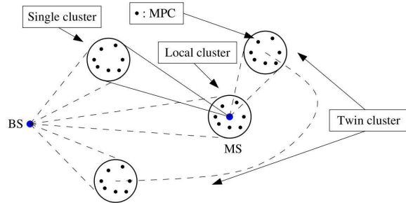
Fig. 9. Three kinds of clusters in COST 2100 channel model [83].
