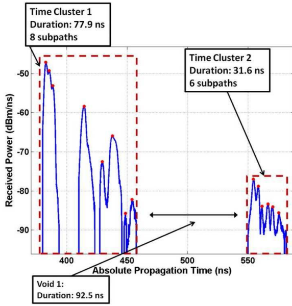
Fig. 7. Measured PDP where two TCs are composed of eight and six subpaths with a 25 ns minimum inter-cluster void interval [70].
