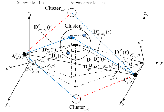
Fig. 15. A general 3D non-stationary 5G GBSM [203].
