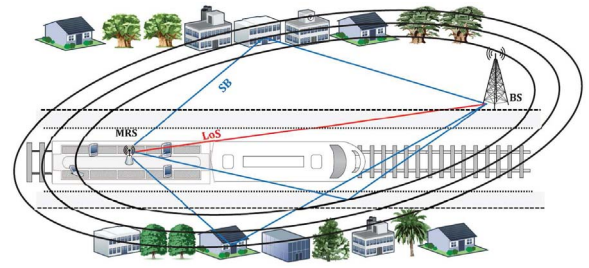
Fig. 5. A multiple confocal ellipses HST channel model [18].
