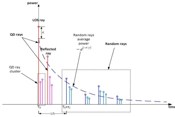
Fig. 10. CIR structure of MiWEBA model [9].
