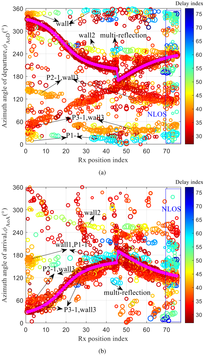
Fig. 11. Angle drifting and cluster evolution along route 1 and route 2. (a) AAoD. (b) AAoA.
