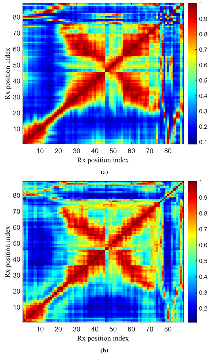
Fig. 12. Multilink correlation of APSD. (a) AoD. (b) AoA.
