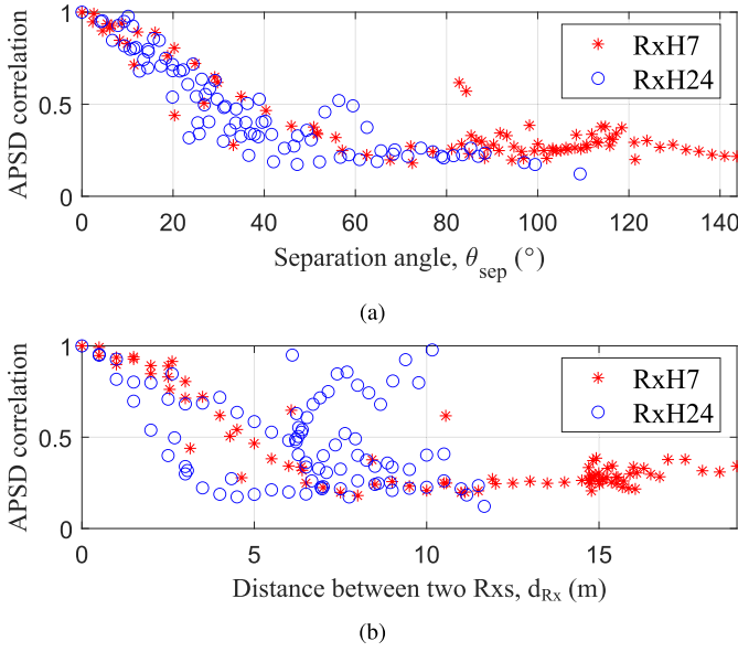
Fig. 13. Multilink APSD correlation of departure angle with \theta_{\text{sep}} and d_{\text{Rx}} at RxH7 and RxH24. (a) Separation angle. (b) Distance between two Rxs.
